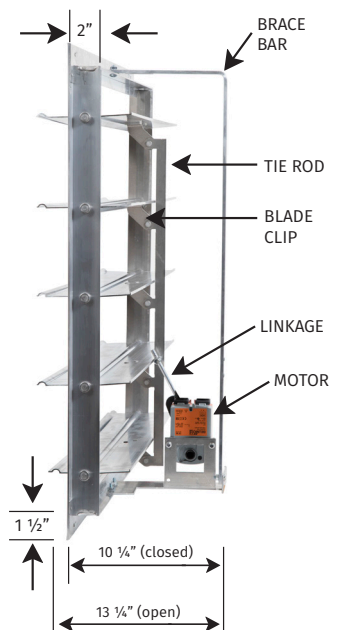
SIDE VIEW (25" to 49")
